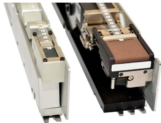
Standard Label Feeder ca. 60 mm
